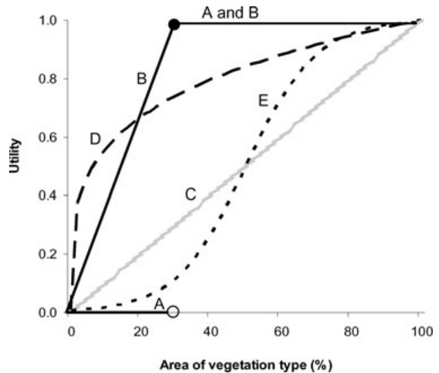
Figure 1 Target-based and alternative utility functions for a single vegetation type. The utility indicates the benefit of protecting increasing amounts of a single vegetation type. (In real-world applications the utility of conserving each of many features, including species and ecosystem services, would be represented by separate functions). In simple binary target-based approaches, utility is zero until the entire target—in this case 30% of the extent of the vegetation type—is reached (A). Alternatively, utility is gained incrementally until the target is reached (B). In both cases, (A and B) no utility is gained beyond the target amount. In contrast, continuous utility functions are never “satiated”: there is always some additional utility from each incremental area protected. They can be linear (C), where utility accrues in equal increments until the entire vegetation type is conserved. Alternatively, they can follow diminishing returns (D) or sigmoidal (E) curves. In these cases, the largest increments of utility are gained where curves are steepest in a positive direction. When curves flatten, efforts are switched to protecting different features for which larger utility can be gained from the same investments.
